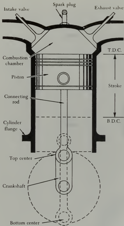
FIGURE 1-25. Components and terminology of engine operation.
